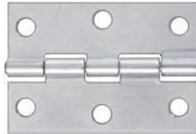
2.5"H x 1.69"W x 0.083" narrow hinge w/removable pin x2
